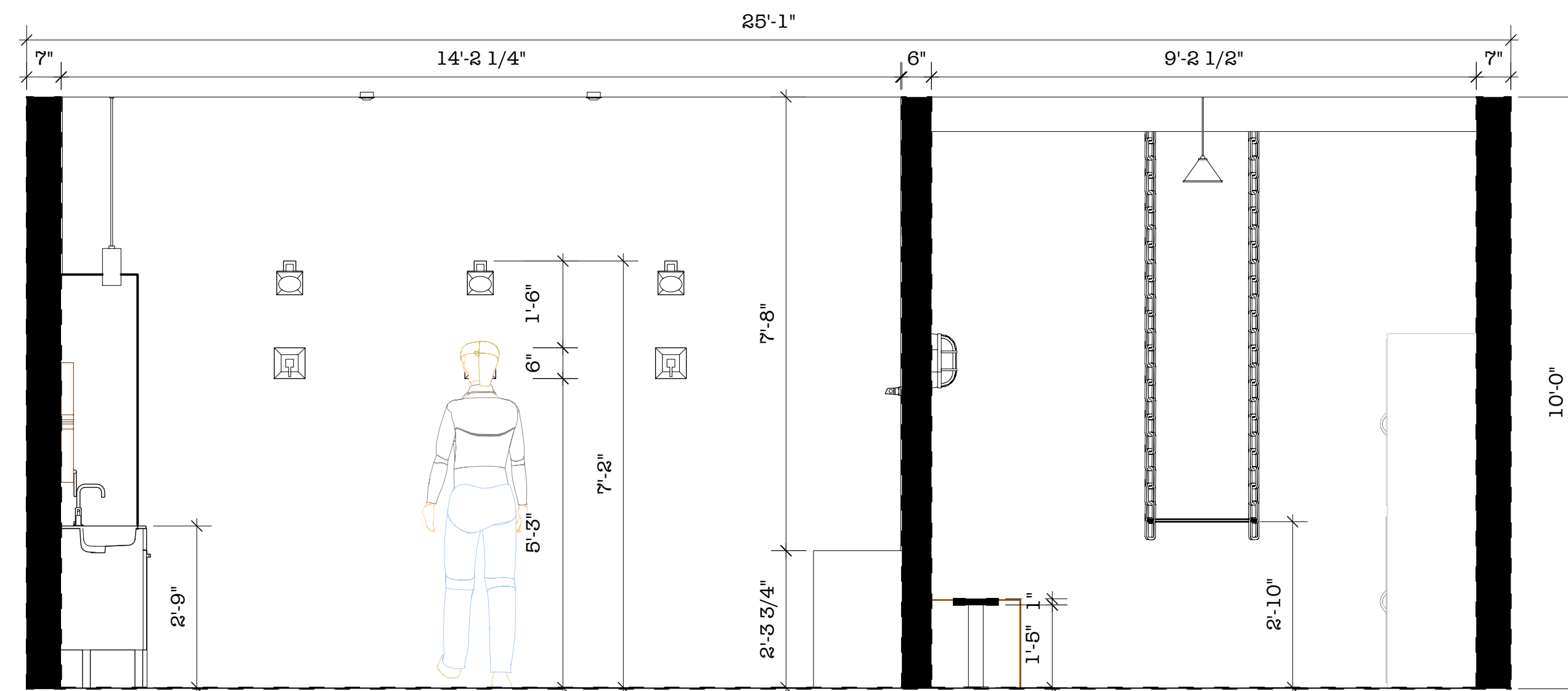
3 Ensuite and Playroom East Scale: 1/2" = 1'-0"
