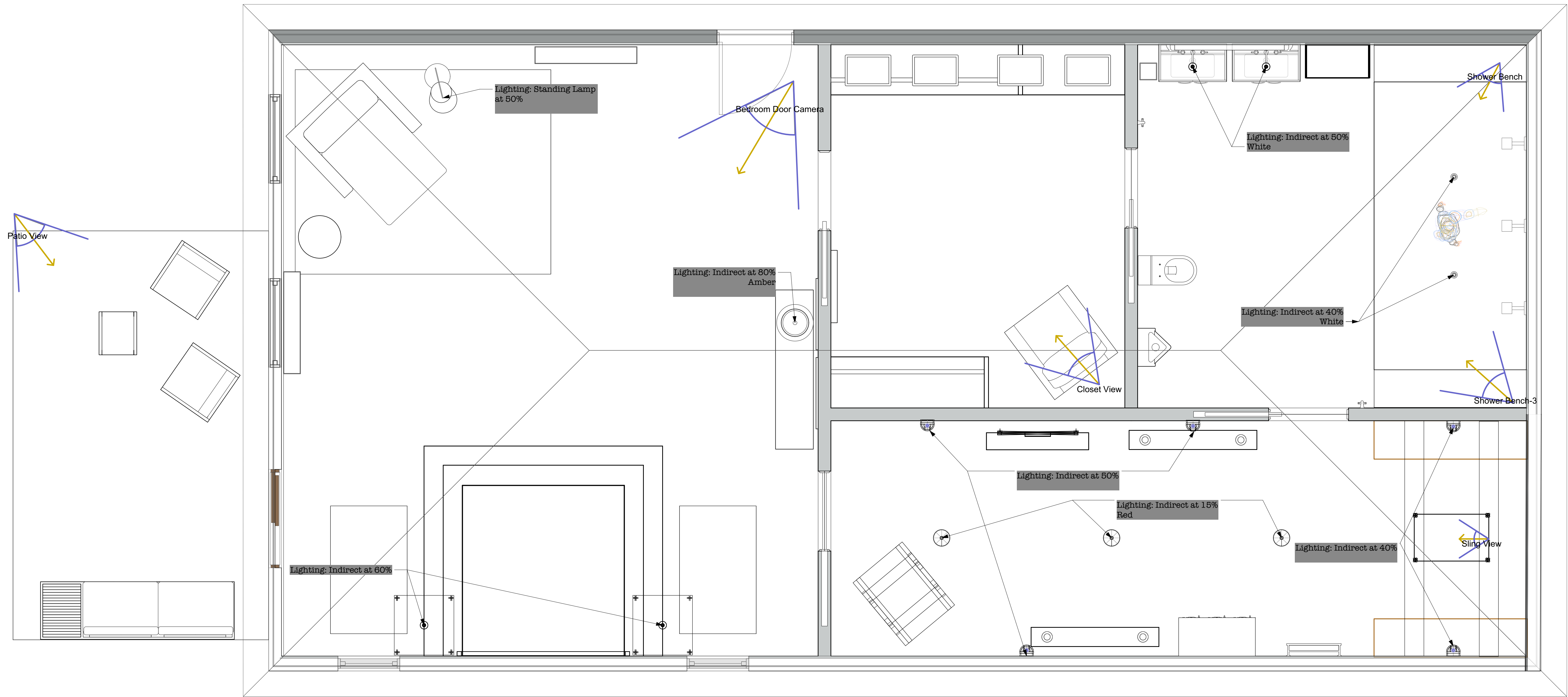
1 Camera and Lighting Plan Scale: 1/2" = 1'-0"
